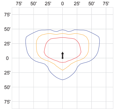
25' Lens Height, 500mA, Type III
