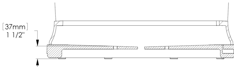
Base casting section view
