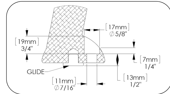
Fig. 1 – Litter leg detail
