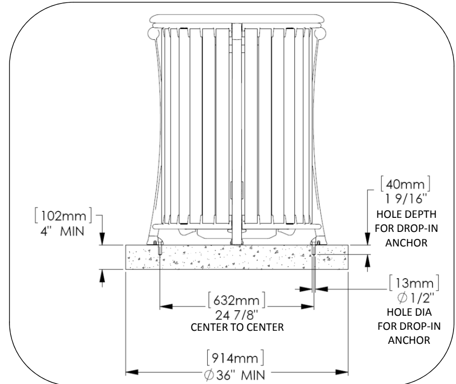
Fig. 2 – Anchor hole details for drop-in anchors
