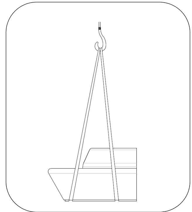
Fig. 1 – Crane install – strap locations
