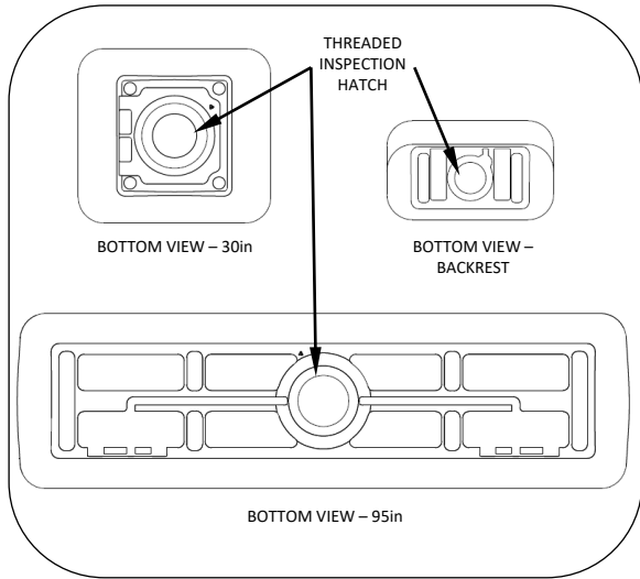
Fig. 1 - anchor components
