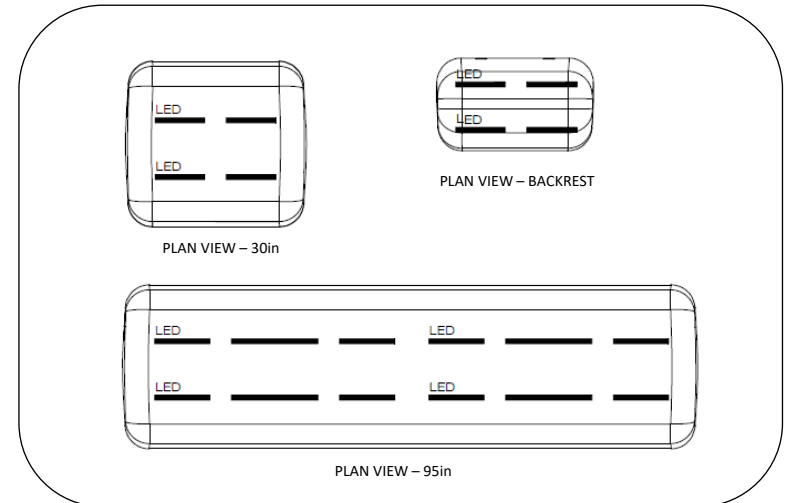
Fig. 4 - LED strip locations, pre-installed (plan view)
